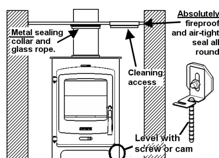
Through steel or concrete closure plate (with cleaning door) into old, oversized, chimney. Steel sealing collar.
