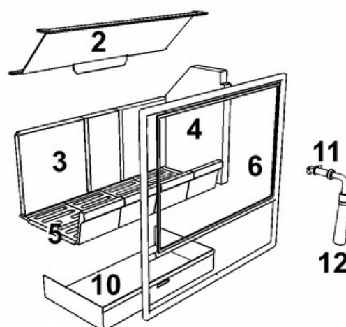
Position of Replaceable Parts (Appearance of each will vary with model)
