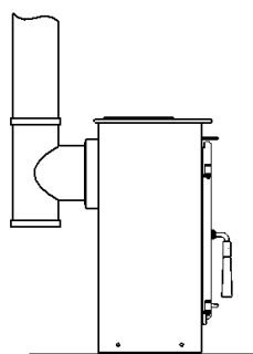
Rear outlet to top outlet by 'T' piece with cleaning door- the preferred method.
