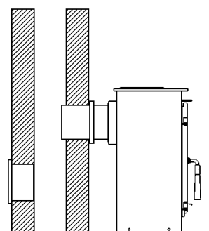
Rear connection into chimney with sealing collar. Cleaning door on opposite side.
