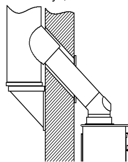
45° top outlet sleeved through wall into external insulated flue. Cleaning hatches on bends.
